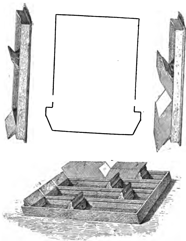
FIG. 119.—Staderini Card Catalogue Trays and Hinged Card (Section 356).
